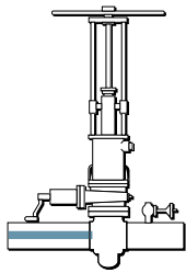
Single stop-off - up to 500psig/34barg/3450kPa
