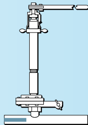
Single stop-off - up to 100psig/7barg/690kPa
