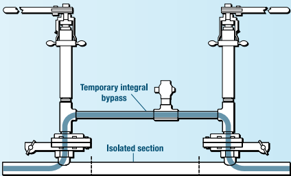
By-pass/double stop-off - up to 100psig/7barg/690kPa
